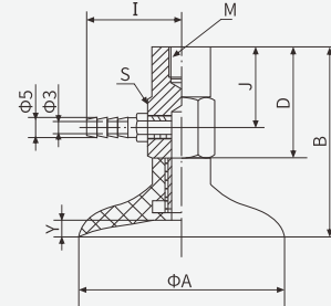
Suction cup diameter: 15-50
