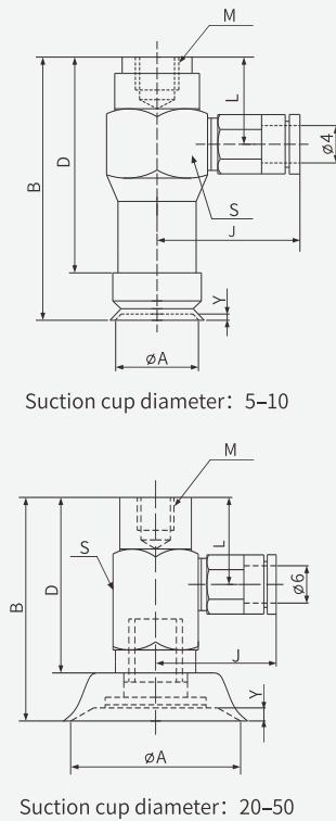
Lateral direction connection - One-touch fitting
