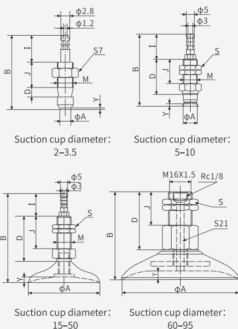
Vertical direction connection-Pagoda fitting
